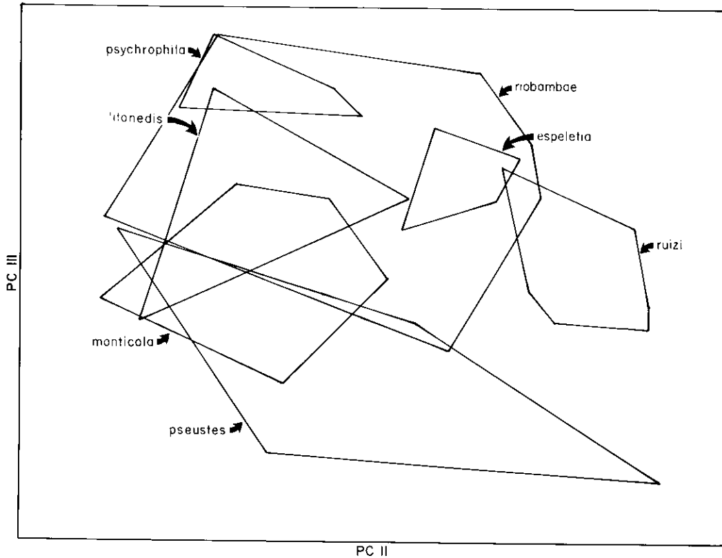
FIG. 2.—Results of a principal components (PC) analysis of morphometric data (16 measurements of 556 specimens) of seven species of Gastrotheca . Axis II is PC II; axis III is PC III.
