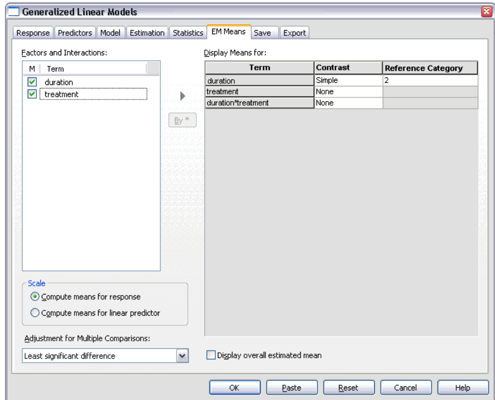
Figure 6-10 Generalized Linear Models: EM Means tab
