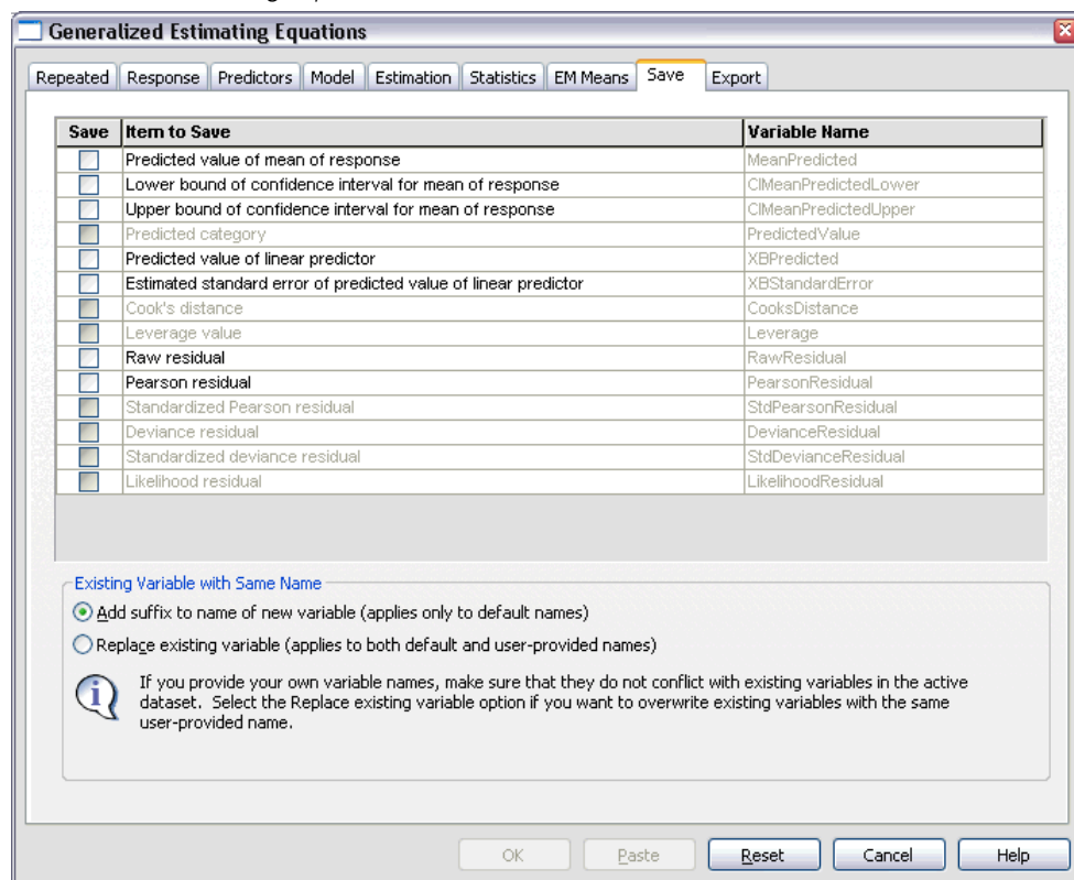
Figure 7-12 Generalized Estimating Equations: Save tab
