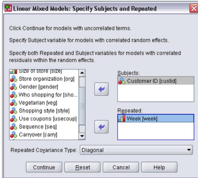
Figure 5-1 Linear Mixed Models Specify Subjects and Repeated Variables dialog box
